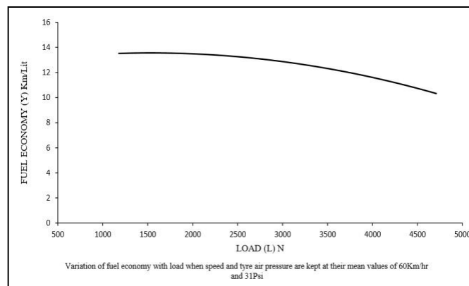
Fig. 3. Outcome of load on fuel economy at mid-levels of speed and tyre air pressure
