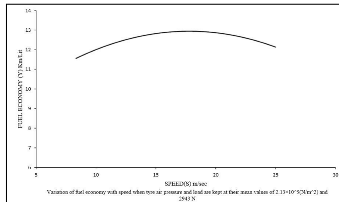
Fig. 1. Outcome of speed on fuel economy at mid-levels of load and tyre air pressure
