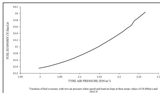
Fig. 3. Outcome of tyre air pressure on fuel economy at mid-levels of speed and load
